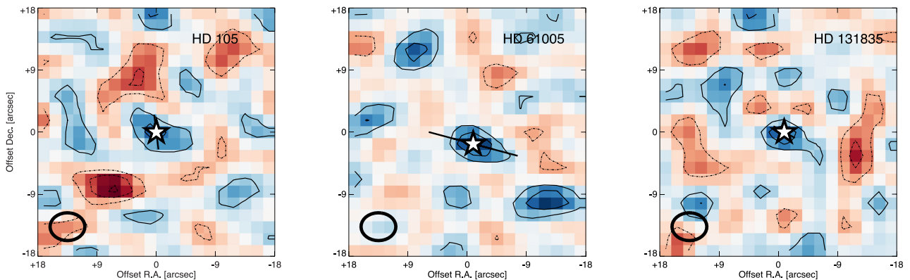
Figure 2. Images of the three debris discs detected in our 9-mm ATCA observations, left to right: HD 105, HD 61005 and HD 131835. The stellar position is denoted by the ‘ \star ’ symbol. The thick solid lines denote the disc extents and position angles, taken from Herschel (HD 105) or scattered light (HD 61005, HD 131835) imaging observations (Hines et al. 2007; Donaldson et al. 2012; Hung et al. 2015). The extension of HD 61005’s disc along the expected position angle is not significant, given the low s/n of the detection. Contours are in 1\sigma increments from \pm 2\sigma and dotted lines denote negative flux. Colour scale is linear from -3\sigma to +3\sigma . The ATCA beam (5 arcsec \times 3 arcsec) is illustrated by the ellipse in the bottom-left corner. Orientation is north up, east left.
